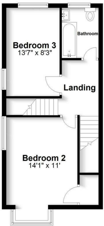
First Floor Approx. 444.0 sq. feet
